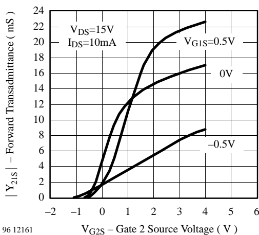
Figure 3. Forward Transadmittance vs. Gate 2 Source Voltage
