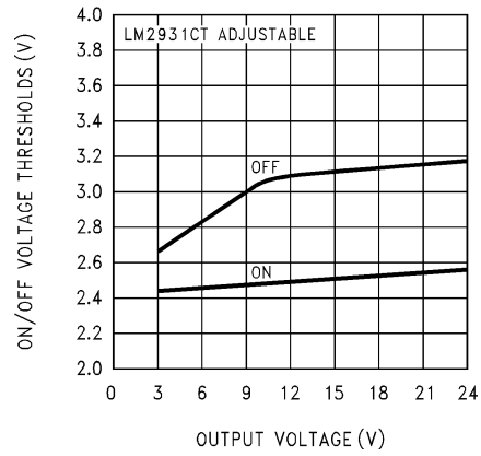
On/Off Threshold
