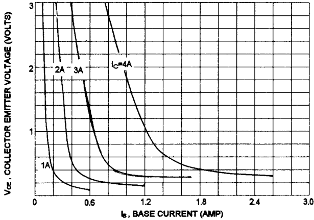
COLLECTOR-EMITTER VOLTAGE
